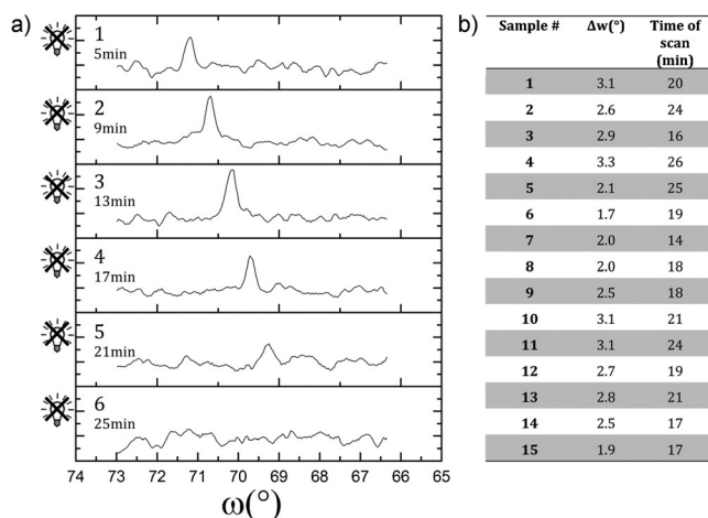
Figure 6. Examples of diffraction spots that disappeared during the light cycle. a) Radially integrated diffraction patterns of one individual diffraction spot in the same experiment as in Figure 5. The \omega of the (012) anhydrous guanine crystal plane shifted when the light was turned off, and the diffraction peak disappeared after a shift of 2.1°. b) Table showing the \Delta\omega [°] of a series of (012) diffraction spots observed in five different fish. The diffraction spots moved in a consistent manner in response to a change in light stimulation, until the diffraction peaks disappeared, when the (012) plane went out of diffraction position. Sample #5 corresponds to the diffraction spot monitored in (a).
