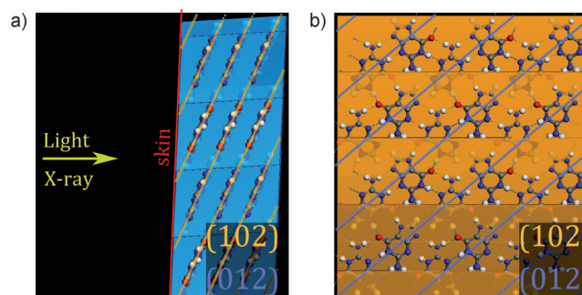
Figure 4. The crystal structure of anhydrous guanine, showing the (102) plane (orange) and the (012) plane (blue). The dihedral angle between the two planes is 68.7°. a) View along the b axis: The crystal (102) plates are edge on to the direction of view. The platelet orientation relative to the fish skin, as well as relative to the incident light and X-ray is indicated; b) View along the a axis: the (012) planes are edge-on to the direction of view. This is the geometry adopted in the diffraction experiment, with the X-ray beam coinciding with the direction of view.
